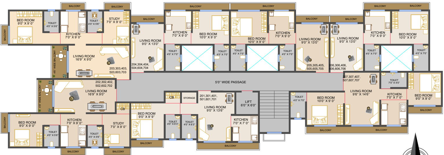
TYPICAL 2ND TO 7TH FLOOR PLAN
